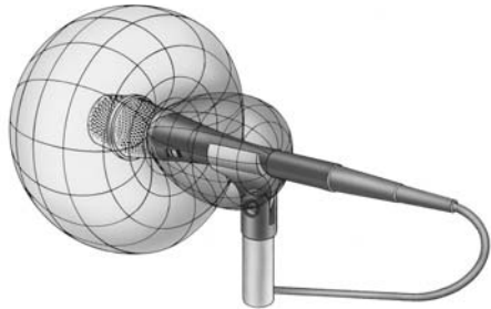
Supercardioid Microphone
